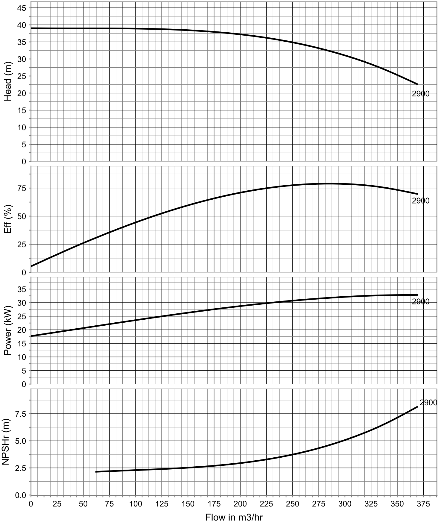
Impeller Dia : 180.0 mm , Stage : 1
