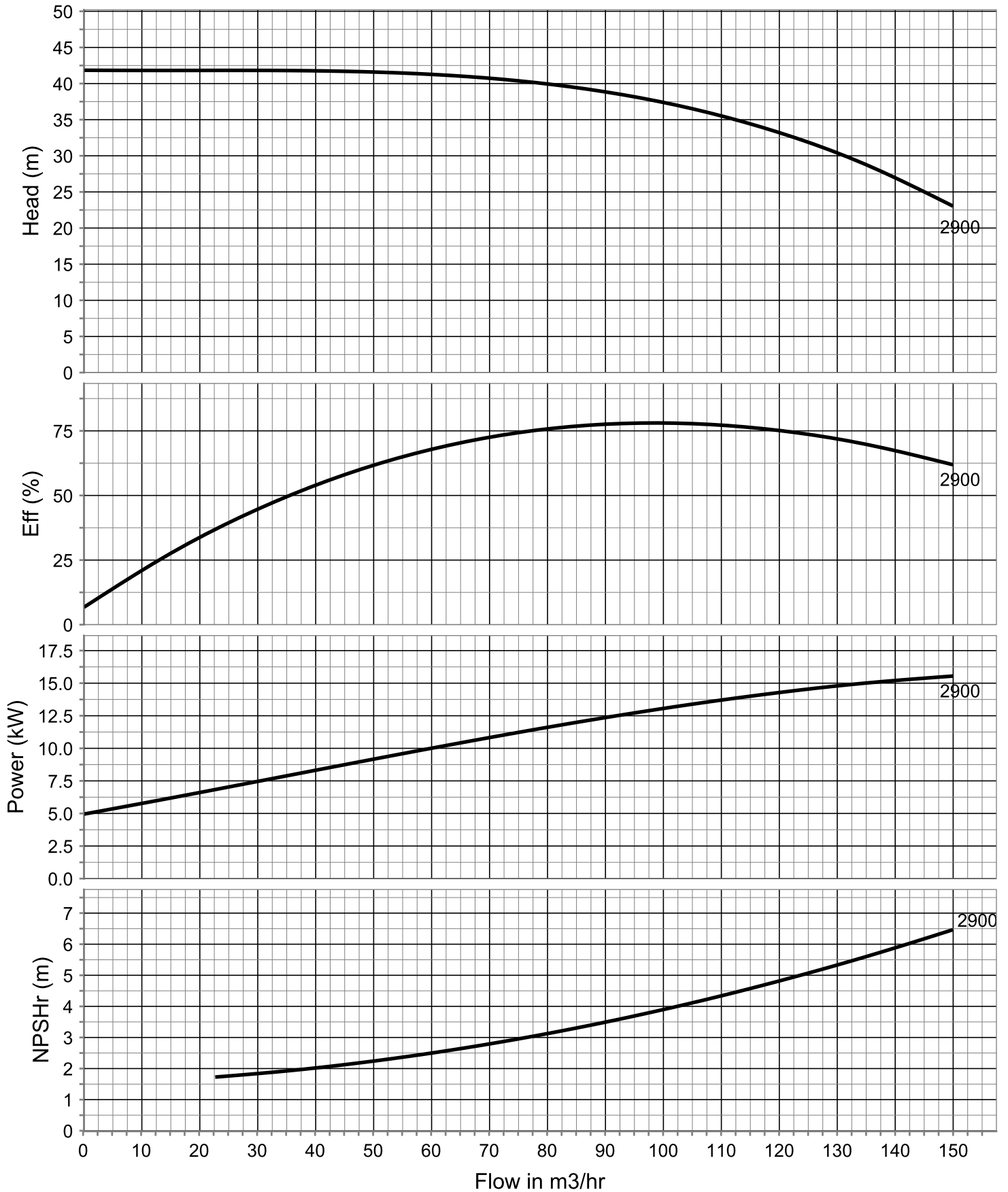
Impeller Dia : 175.0 mm , Stage : 1
